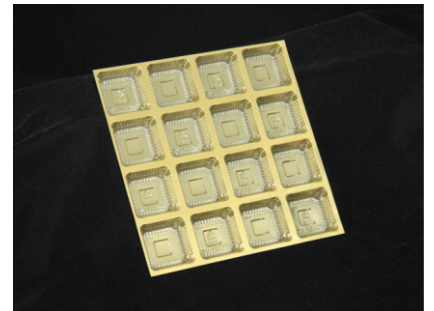
O-Series 16 Cavity
