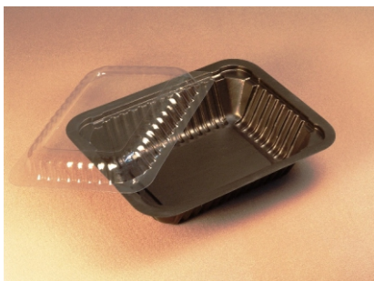
Item: MITA® 002-1813 Outer Size Tray (mm): 185 x 155 x 45 Inner Size Tray (mm): 180 x 130 Total Height With Lid (mm): 60
